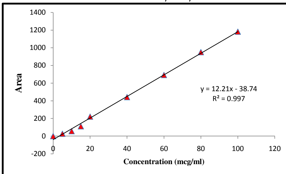
Figure 4: Linearity Plot
